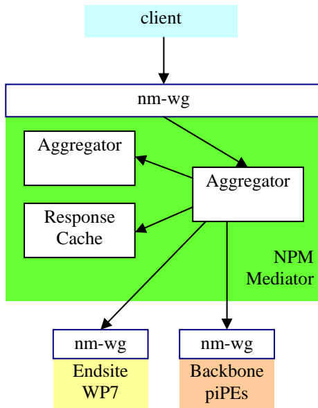
Figure 5: Mediator internals
