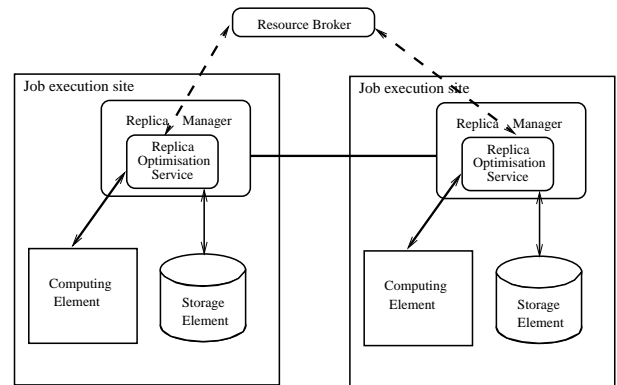
Figure 1. European DataGrid Architecture.
